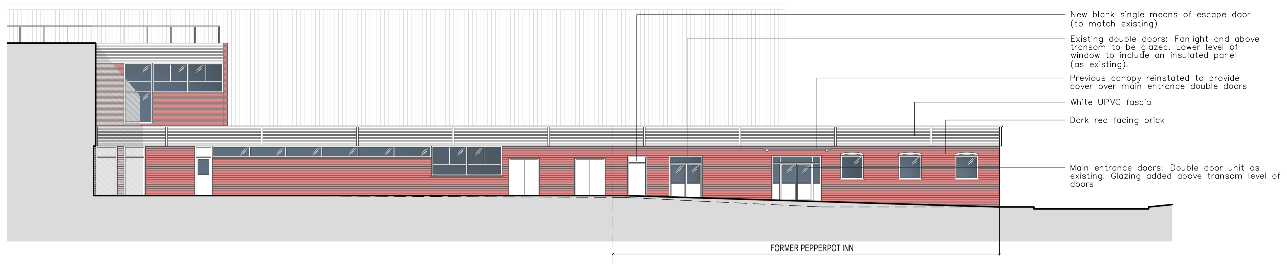
ELEVATION A (FRONT) AS PROPOSED SCALE - 1:100
