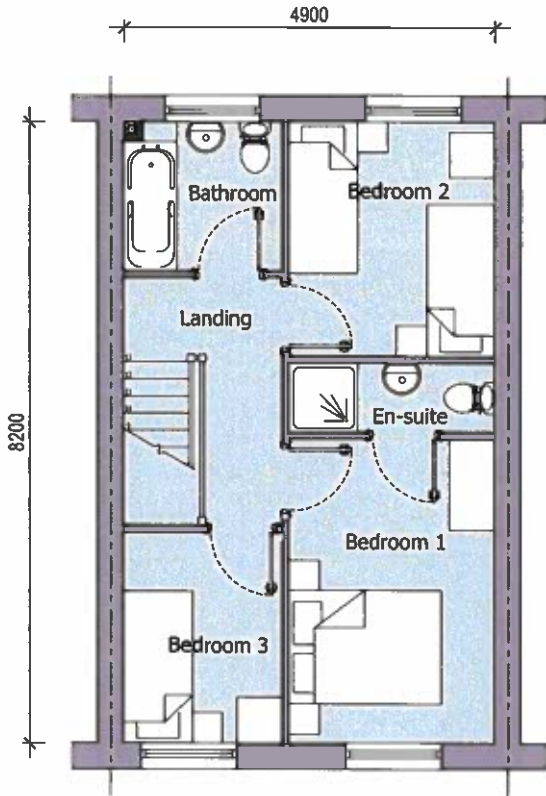
FIRST FLOOR PLAN (terrace) 3B5P HOUSE FLOOR AREA = 40.18m 2 SCALE 1:100
