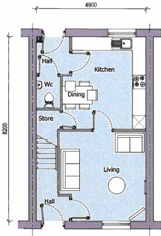
GROUND FLOOR PLAN (terrace) 3B5P HOUSE FLOOR AREA = 40.18m 2 SCALE 1:100
